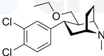
Tesofensine Structure (C 17 H 23 Cl 2 NO MW: 328.28)
