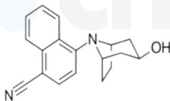
Fig.1. Structure of AC262 (C 18 H 18 N 2 O : MW: 278.2)
