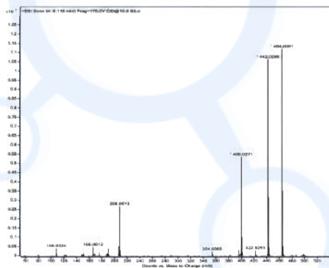
Fig. 1. Spectrum and Chromatography of LCMS/MS
