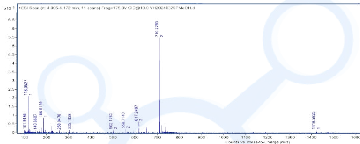
Fig.1. MS spectrum of BPC-157 in capsule
